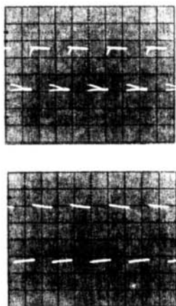
Fig.3 Differential Measurements
