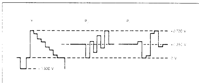
SMPTE/EBU component standard, 100% amplitude color bar signal. P_b and P_r offset by +350 mV to match luminance range.
