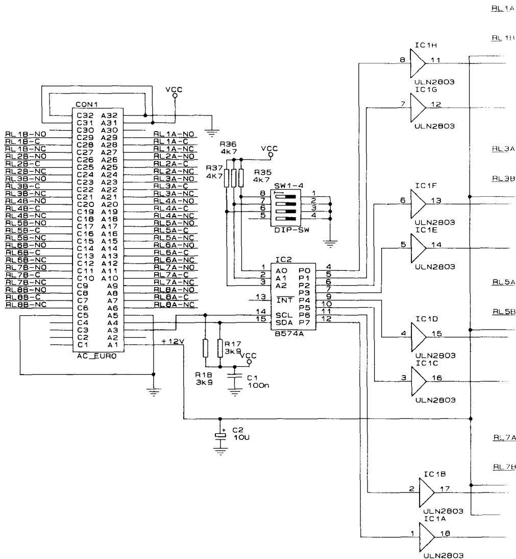
I 2 C Relay Board Circuit Diagram
