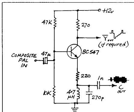
Fig.3 Chroma-Luma separation
