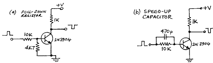
Fig.2 Preventing Pulse-lengthening
